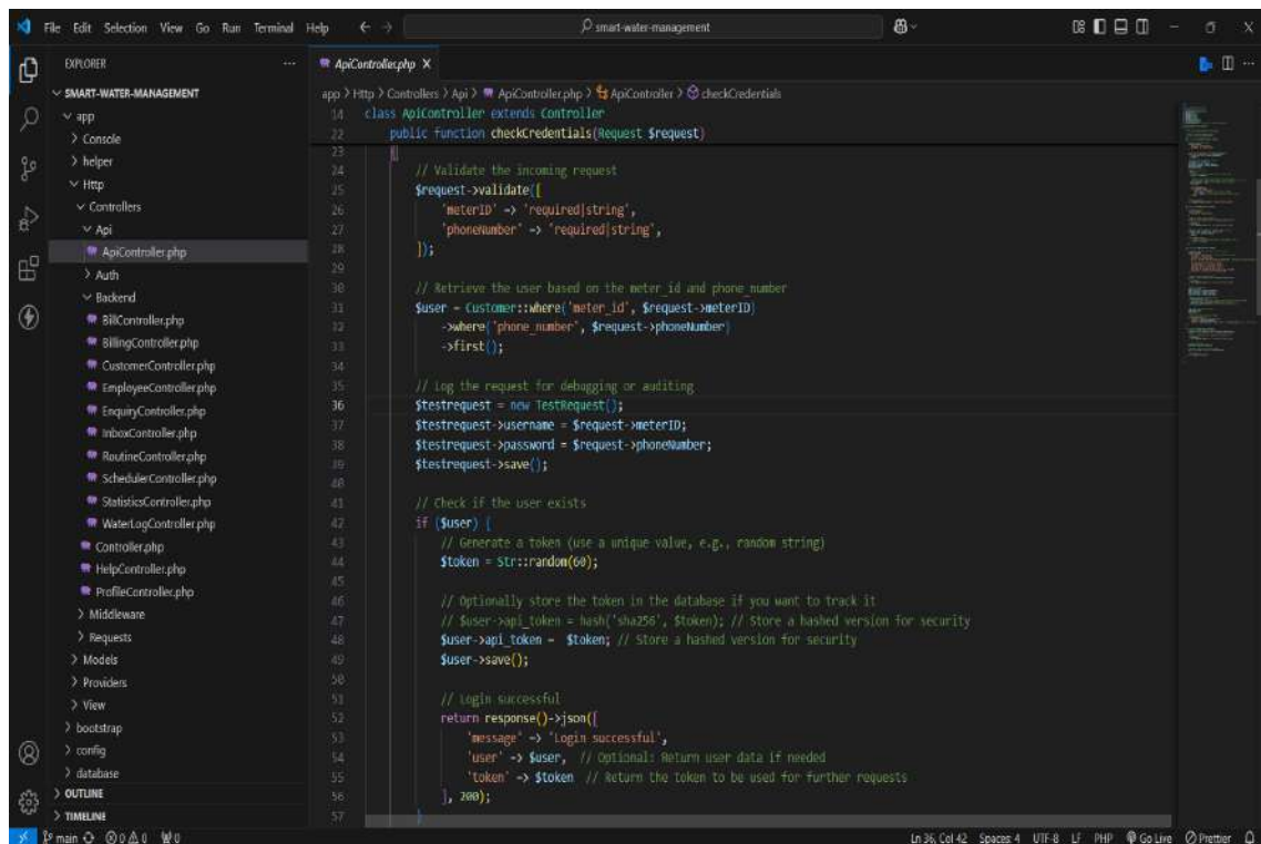
Figure 7.1: API Controller
