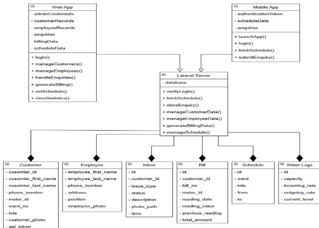
Figure 4.1: Class Diagram
