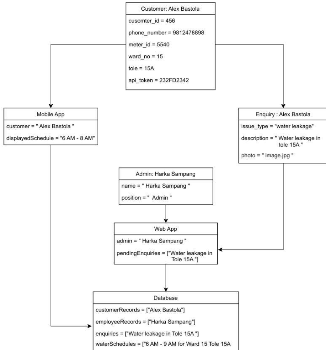
Figure 3.2: Object modeling
