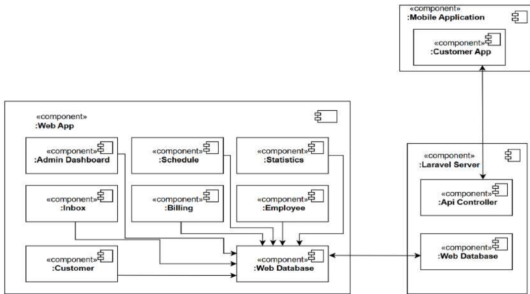
Figure 4.5: Component Diagram
