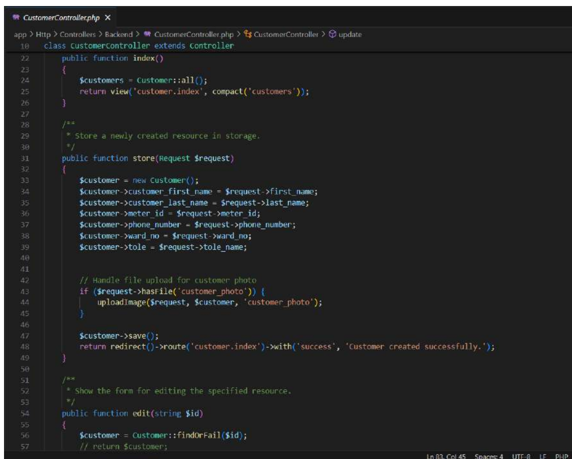
Figure 7.2: Customer Controller
