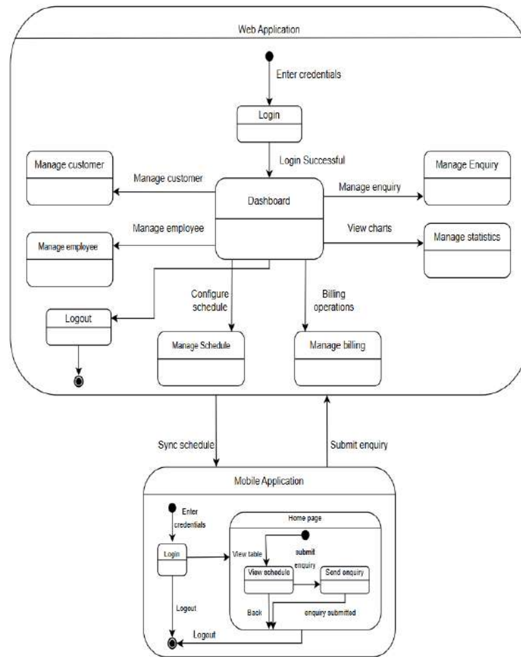
Figure 4.4: State Diagram
