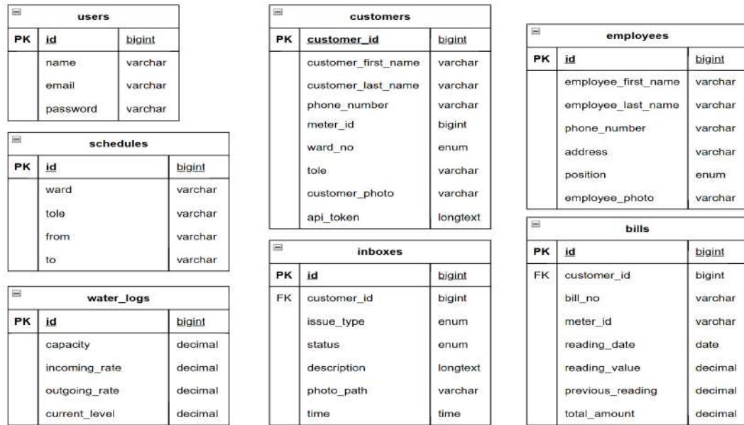
Figure 4.2: Database Schema
